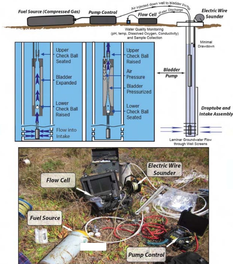
Figure 4. Low Flow Groundwater Sampling System Presented in Cartoon and Photograph
