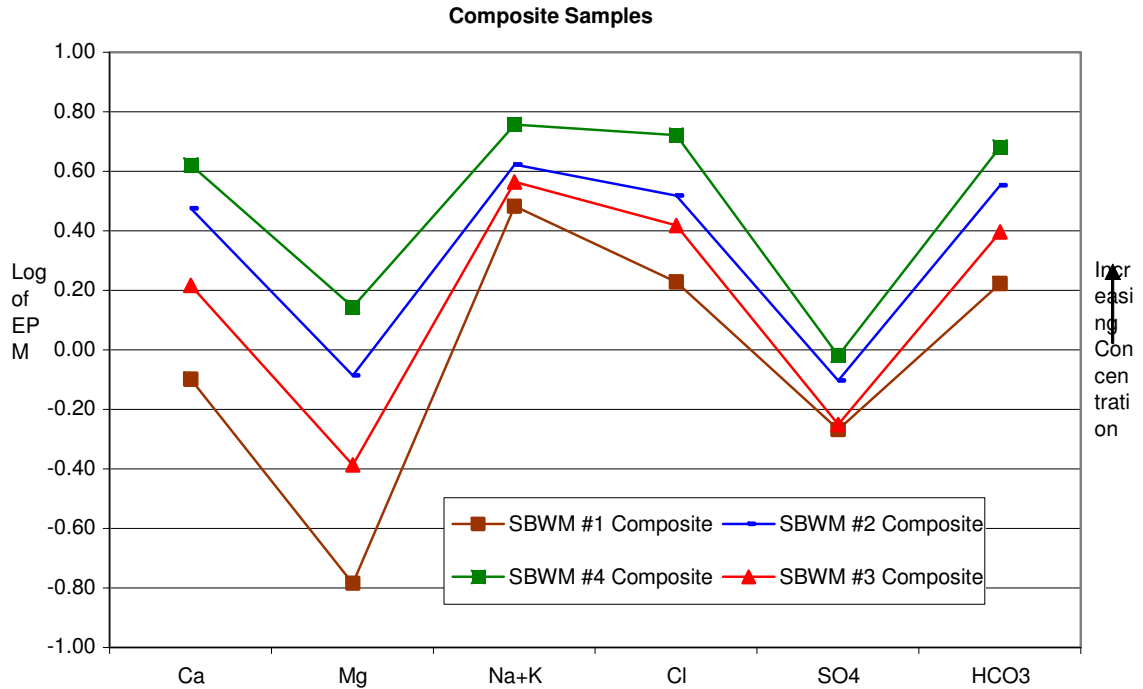
Figure 5. Graphs of Water Quality Samples
