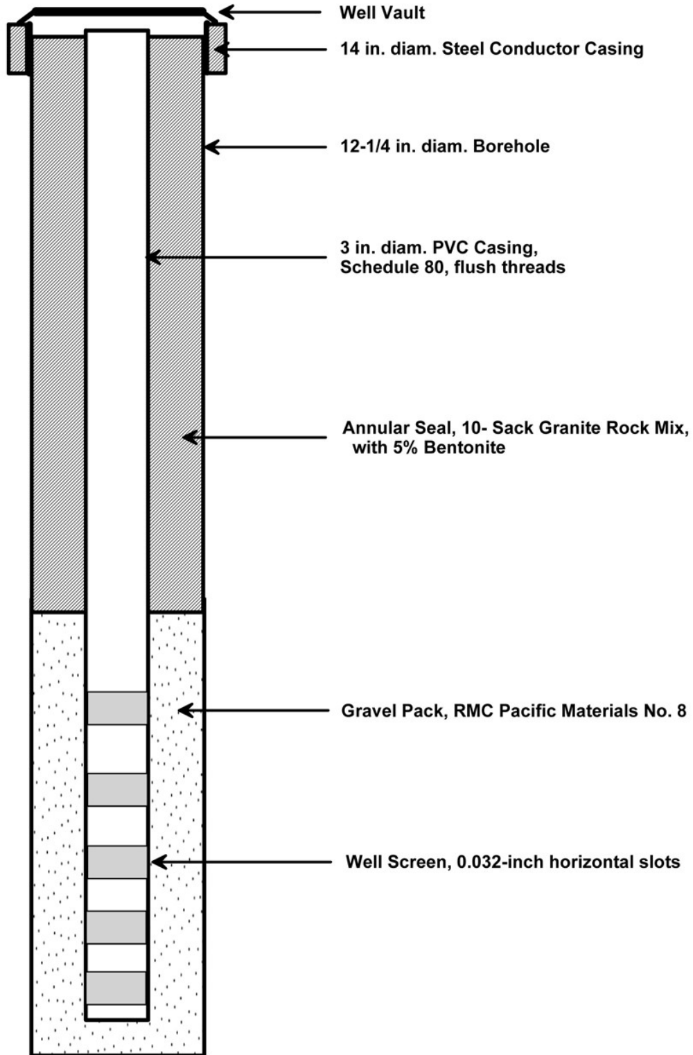
Figure 2. Typical Sentinel Well Construction
