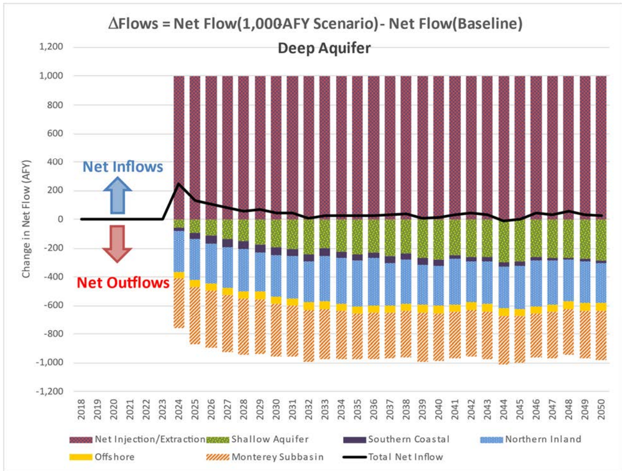
Figure 13. Deep Aquifer: Change in Net Flows between Baseline and 1,000-AFY Replenishment Scenarios
