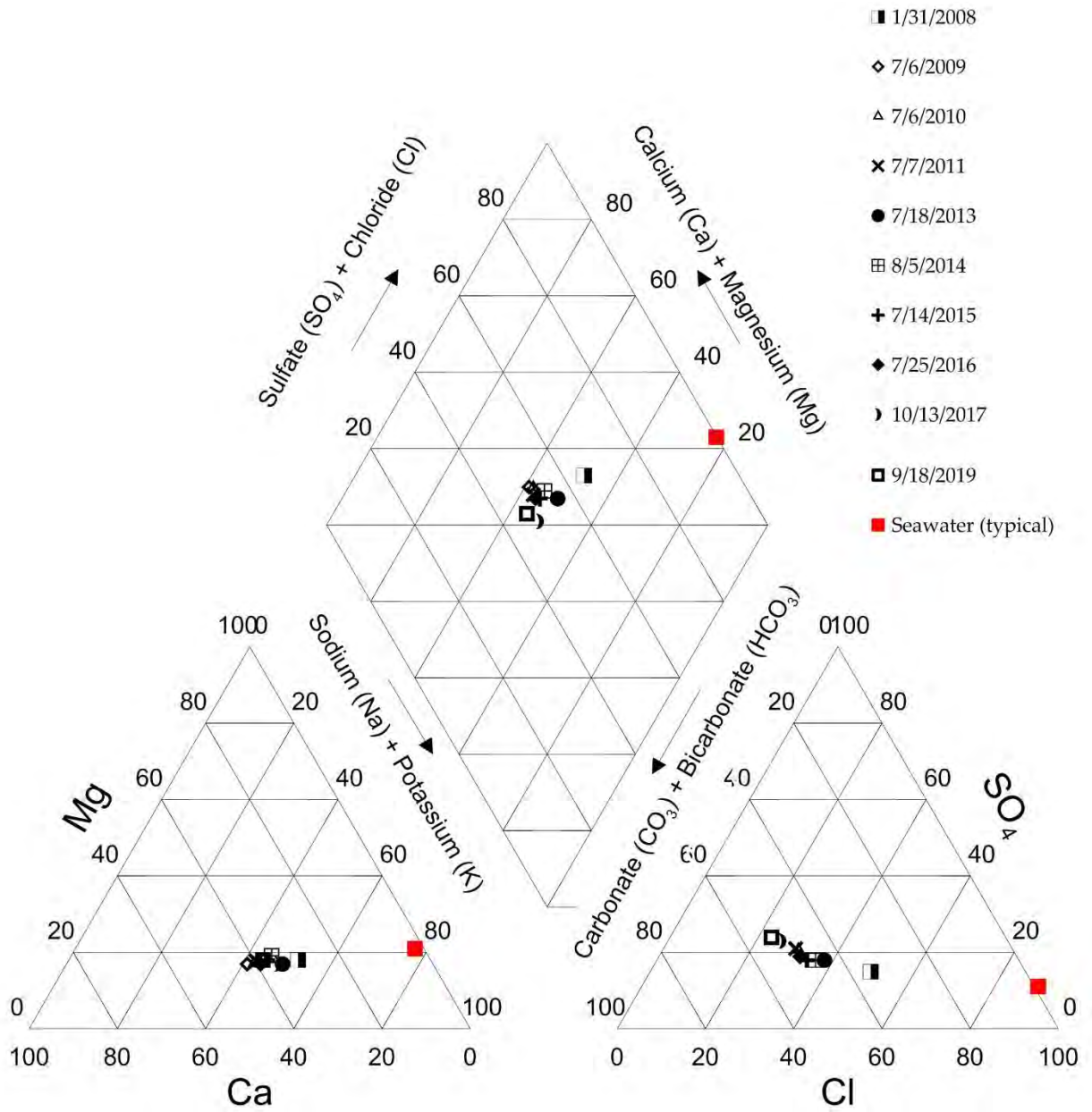
Figure C-28. Piper Diagram of Paralta Production Well
