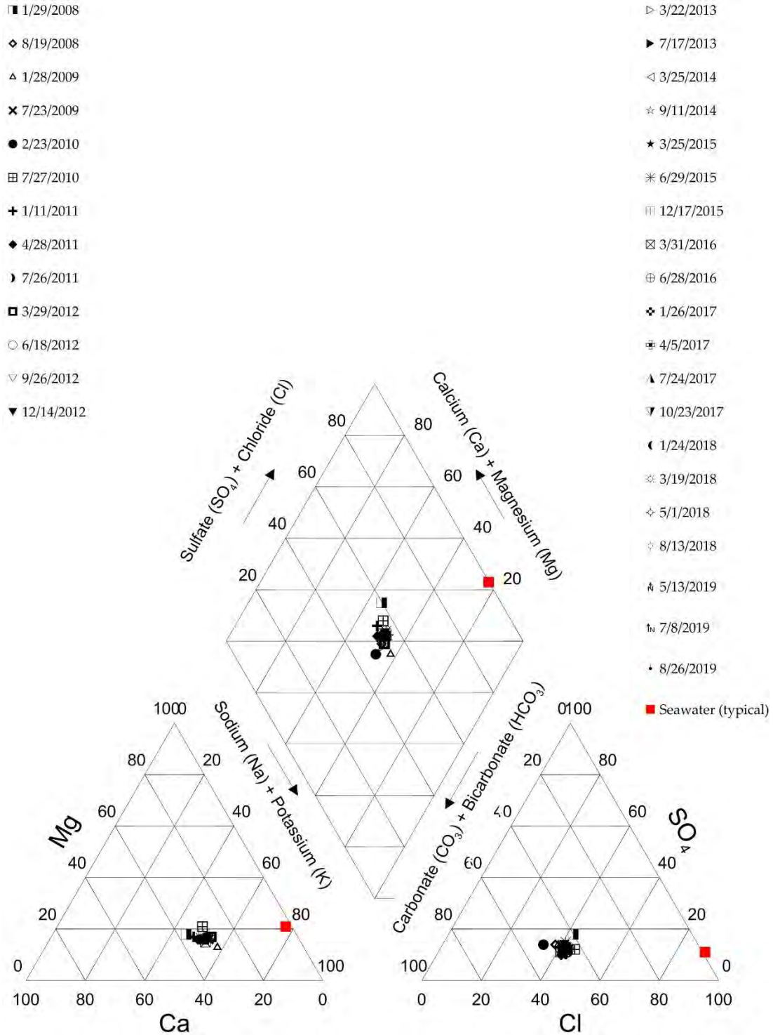
Figure C-7. Piper Diagram of MSC Shallow
