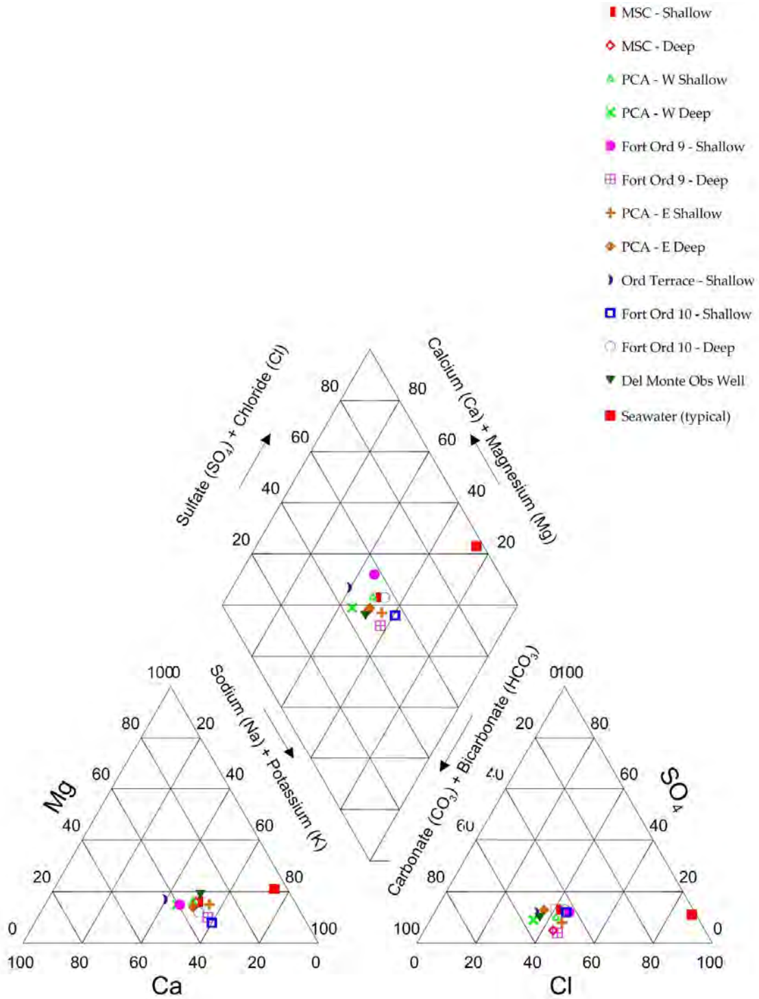
Figure 15: Piper Diagram for Seaside Groundwater Basin Monitoring Wells, 4 th Quarter Water Year 2018 (July- September 2018) (Data source: Watermaster)
