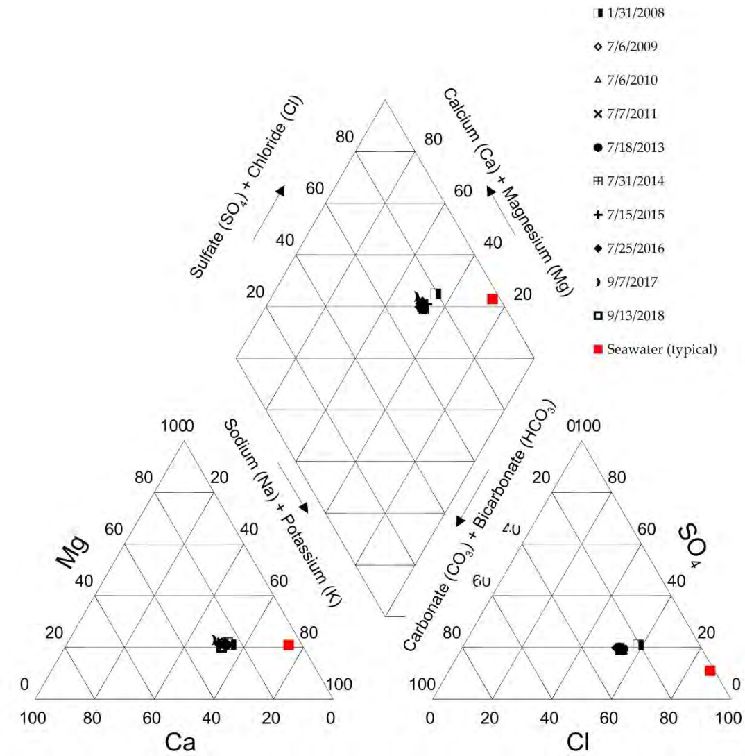
Figure A-16: Piper Diagram of Plumas 4 Production Well
