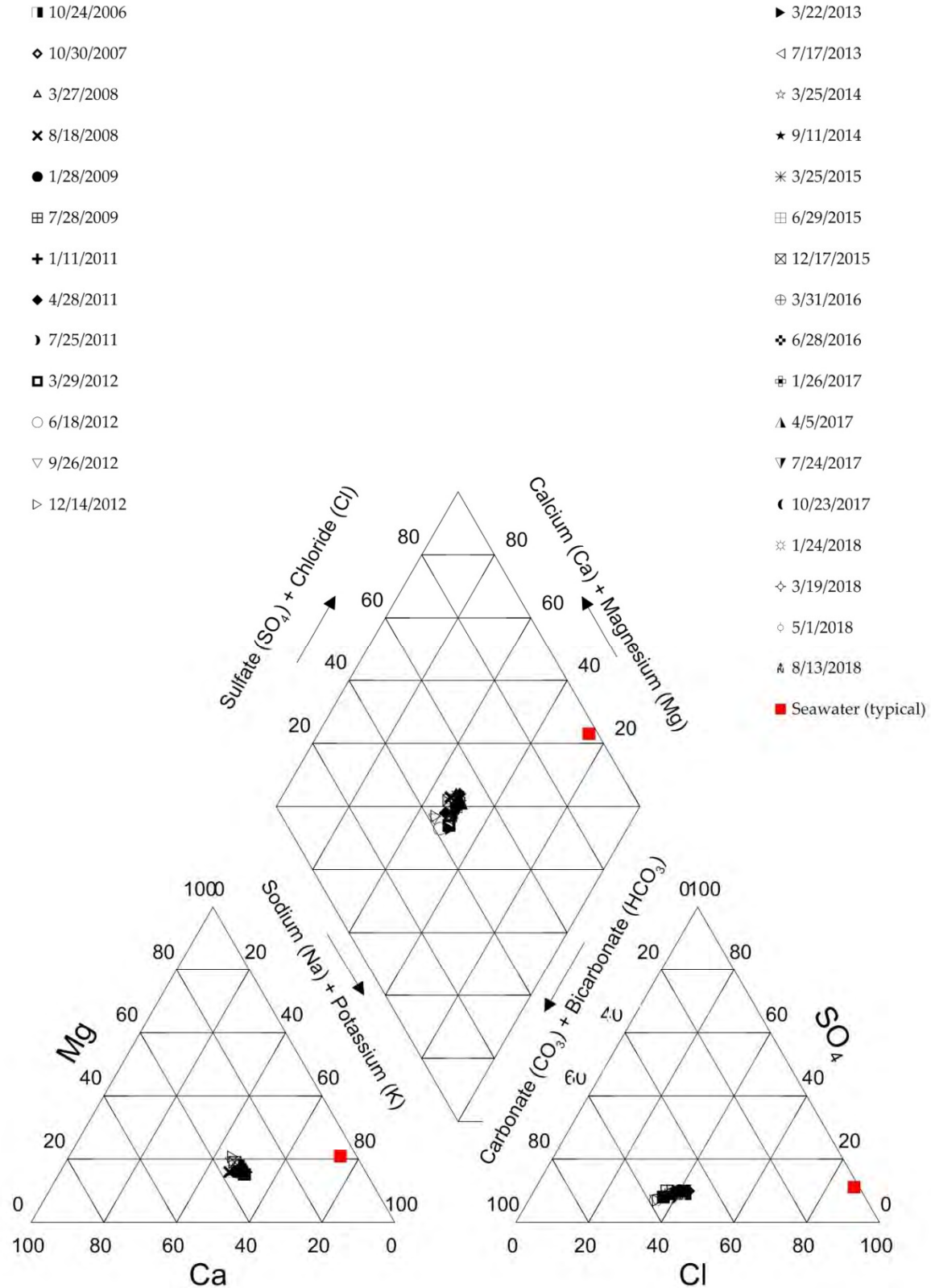
Figure A-1: Piper Diagram of PCA West Shallow
